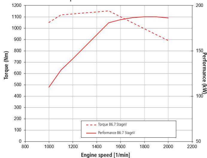
Torque and Performance PB 100
