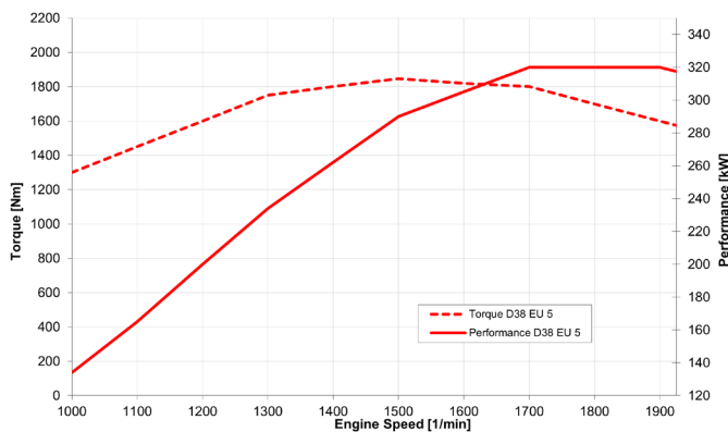
Power and torque L9 EU StageV
