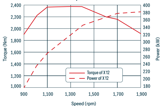
Power and torque of Cummins X12
